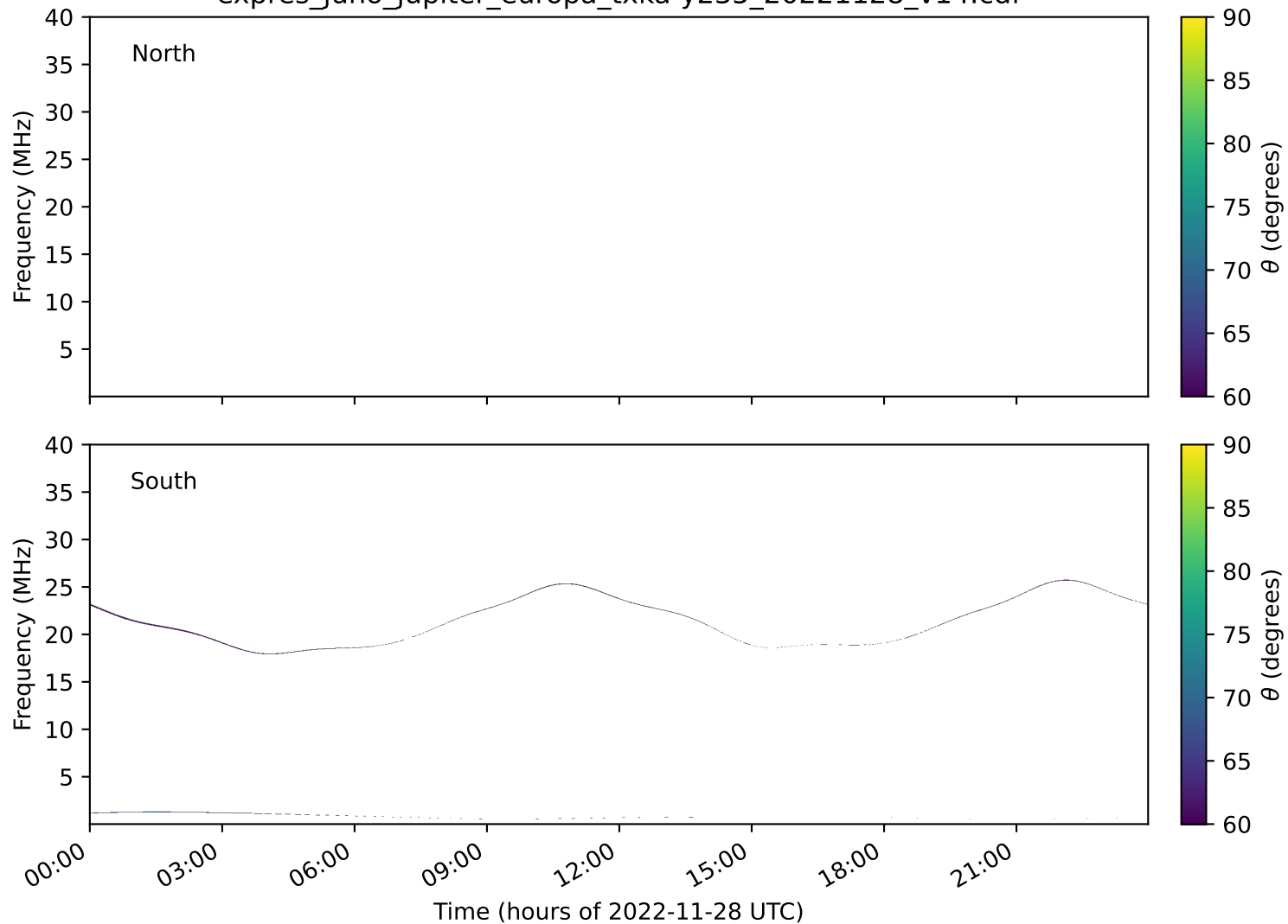
expres_juno_jupiter_europa_txka-y235_20221128_v14.cdf
