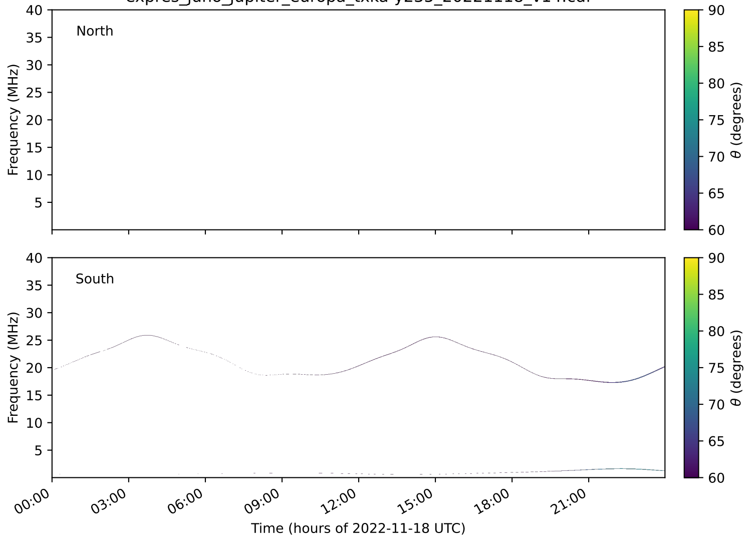
expres_juno_jupiter_europa_txka-y235_20221118_v14.cdf
