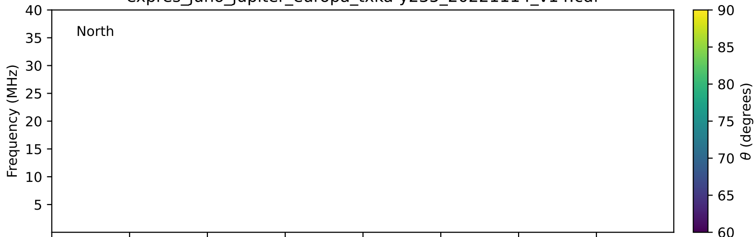
expres_juno_jupiter_europa_txka-y235_20221114_v14.cdf
