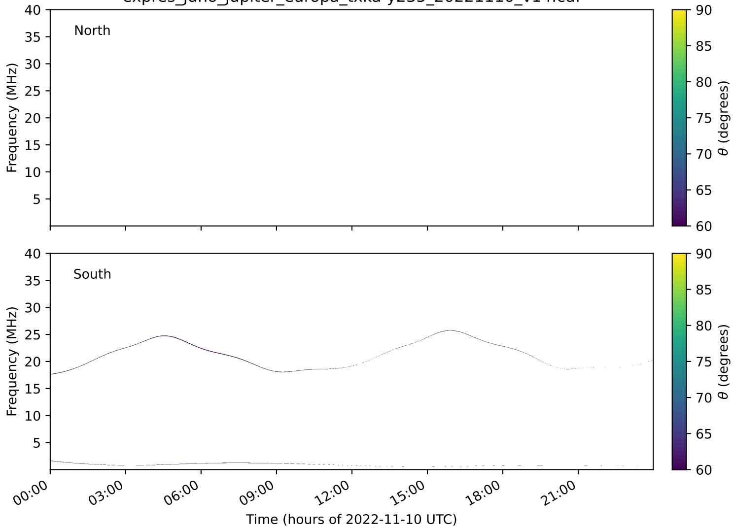
expres_juno_jupiter_europa_txka-y235_20221110_v14.cdf
