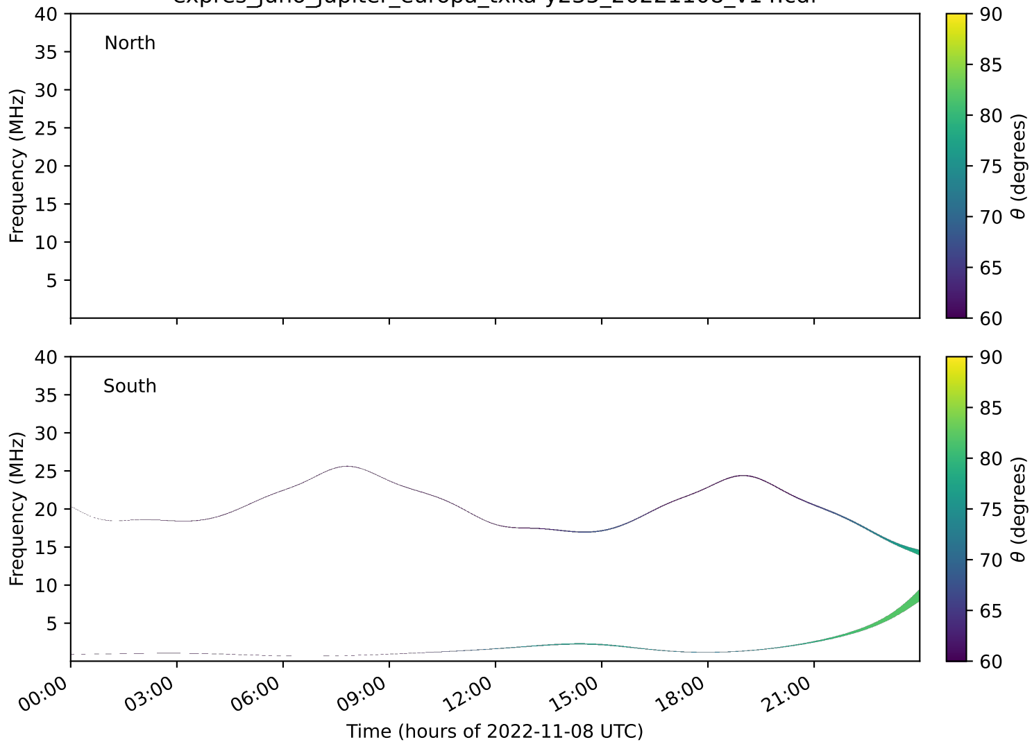
expres_juno_jupiter_europa_txka-y235_20221108_v14.cdf
