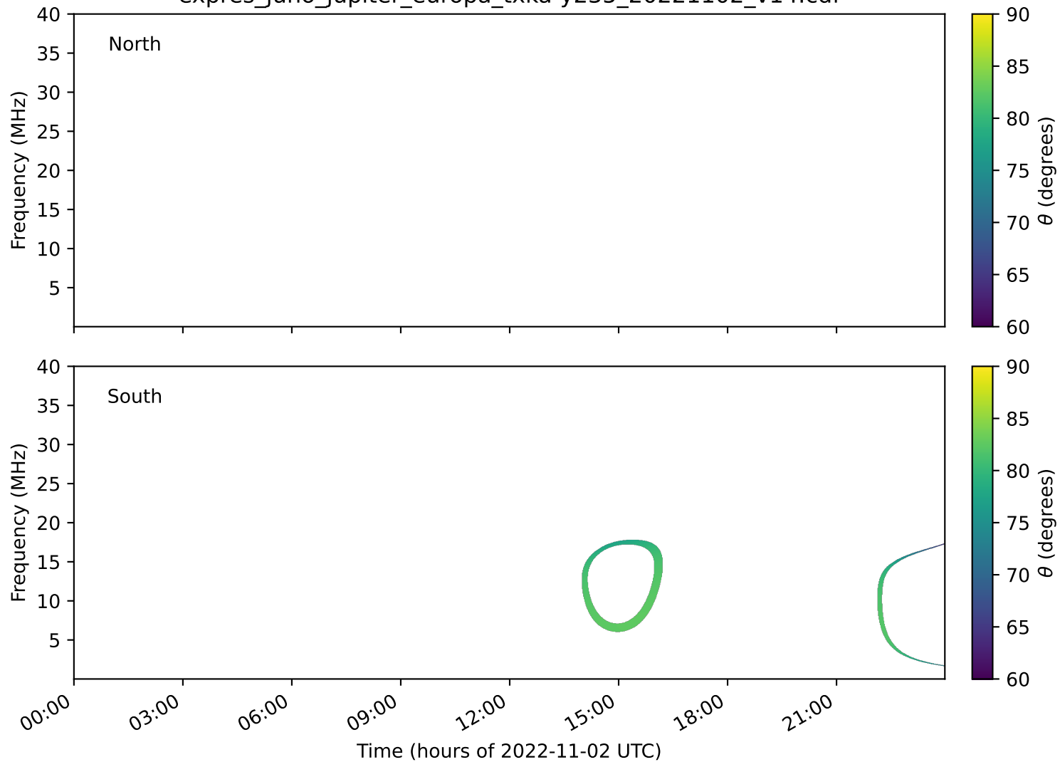
expres_juno_jupiter_europa_txka-y235_20221102_v14.cdf
