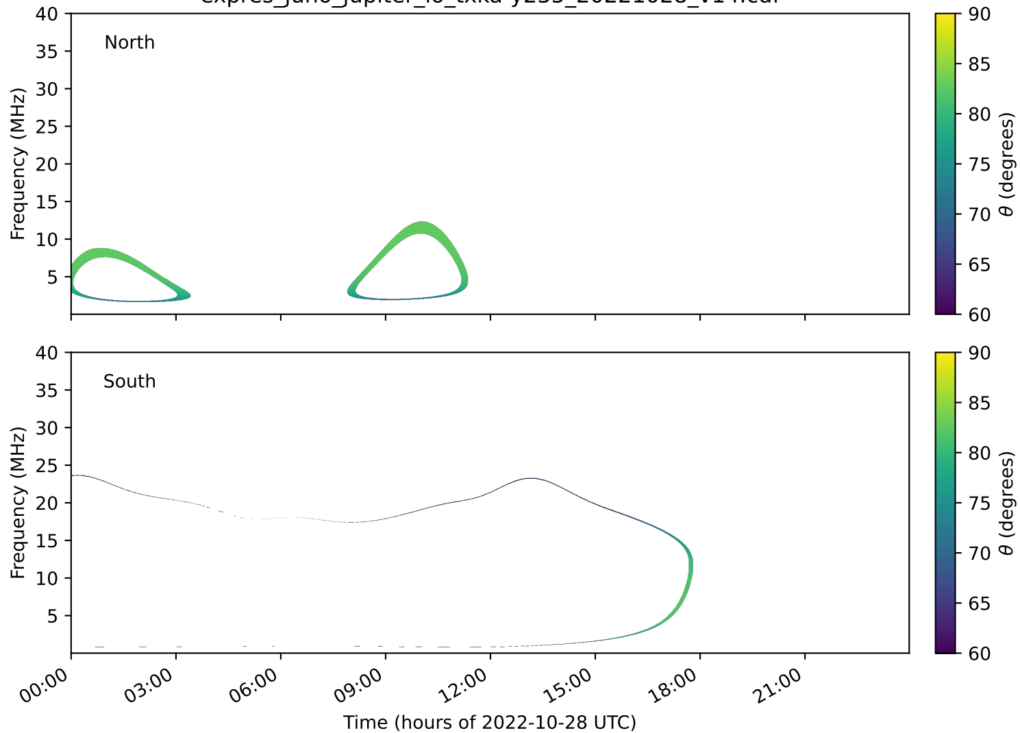
expres_juno_jupiter_io_txka-y235_20221028_v14.cdf
