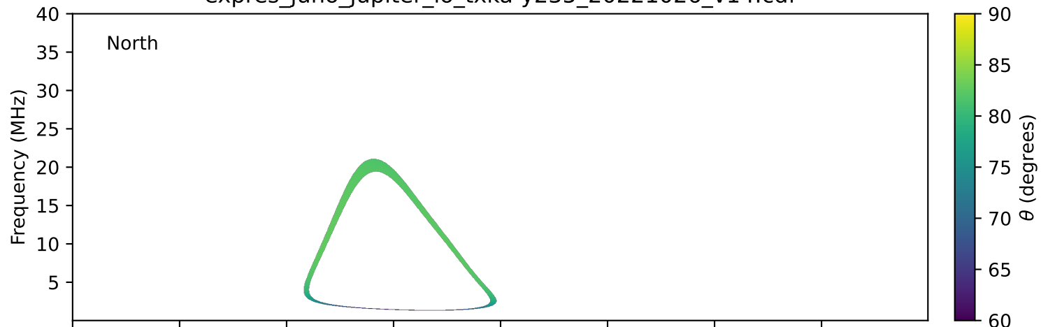
expres_juno_jupiter_io_txka-y235_20221026_v14.cdf
