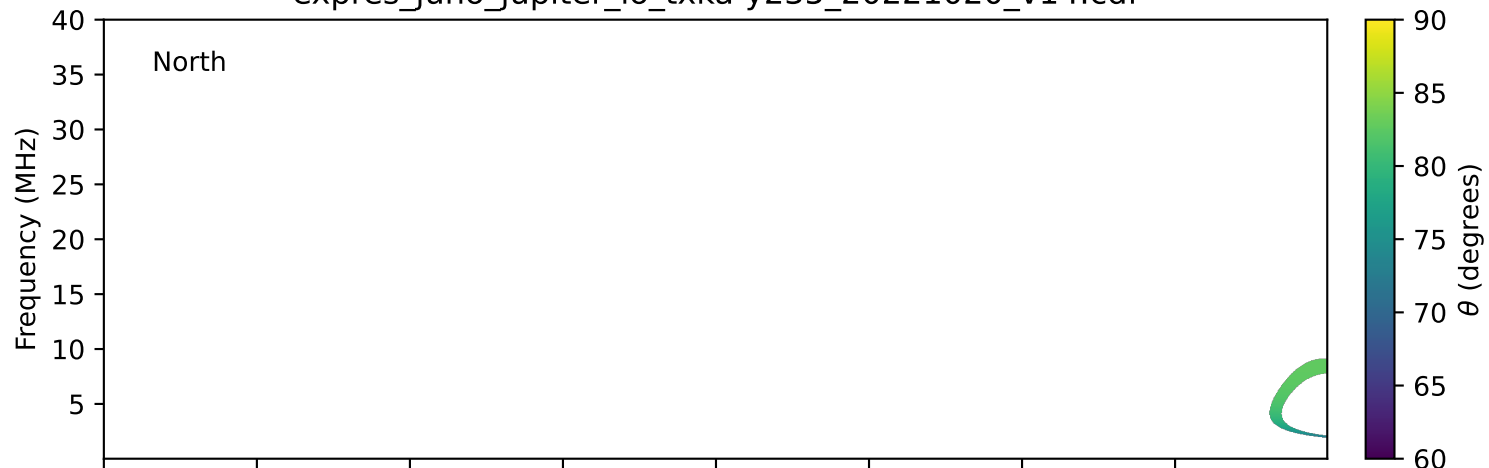
expres_juno_jupiter_io_txka-y235_20221020_v14.cdf
