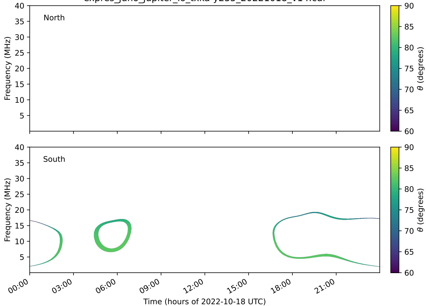
expres_juno_jupiter_io_txka-y235_20221018_v14.cdf
