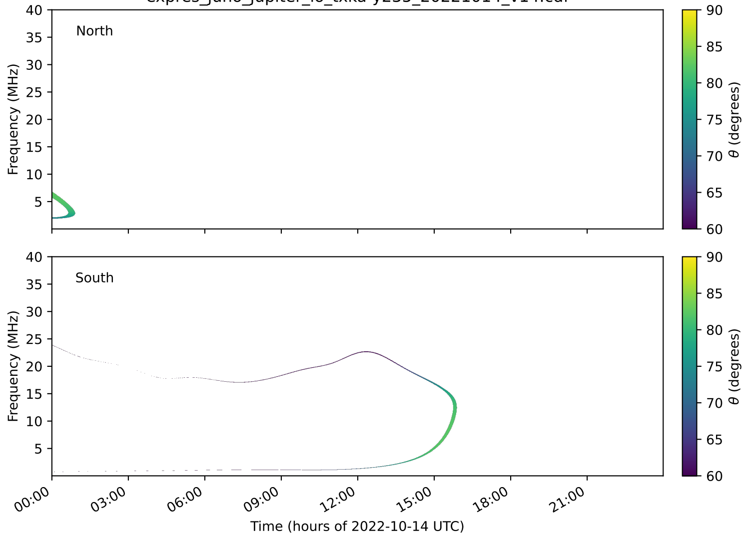
expres_juno_jupiter_io_txka-y235_20221014_v14.cdf
