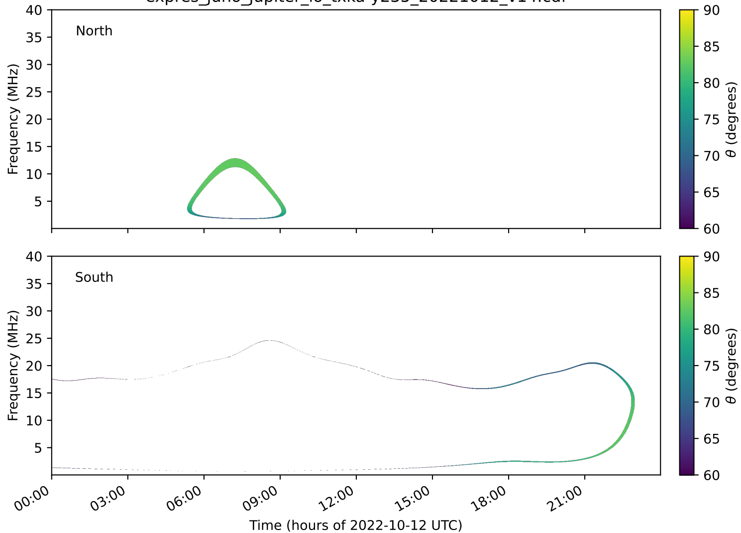
expres_juno_jupiter_io_txka-y235_20221012_v14.cdf
