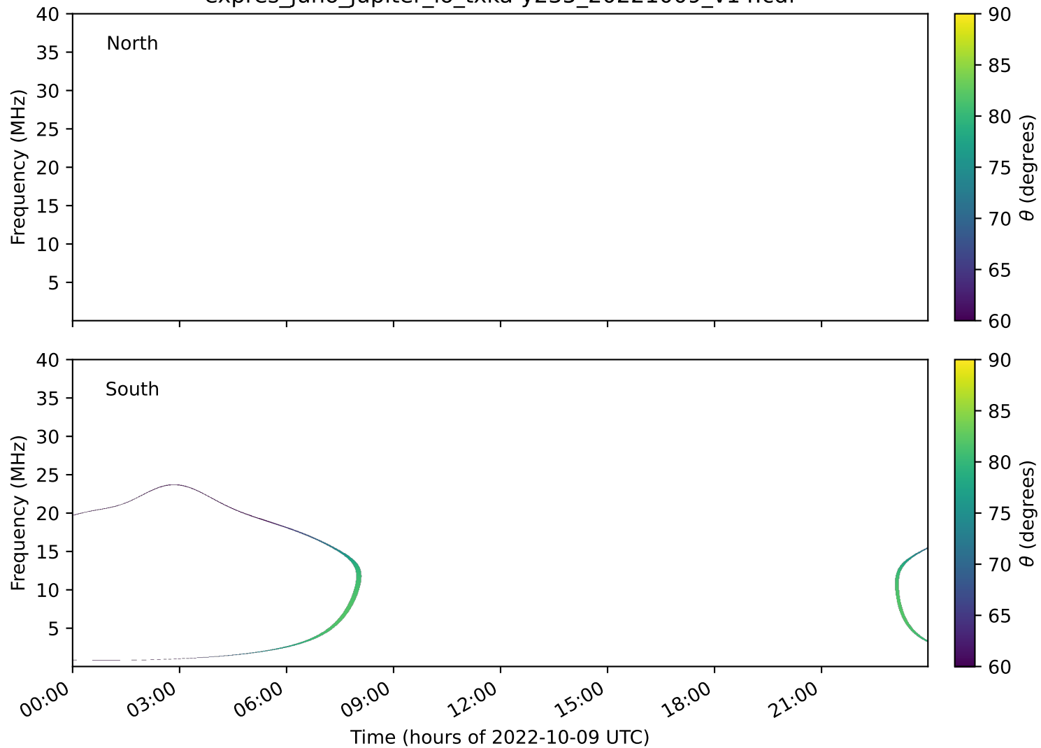
expres_juno_jupiter_io_txka-y235_20221009_v14.cdf
