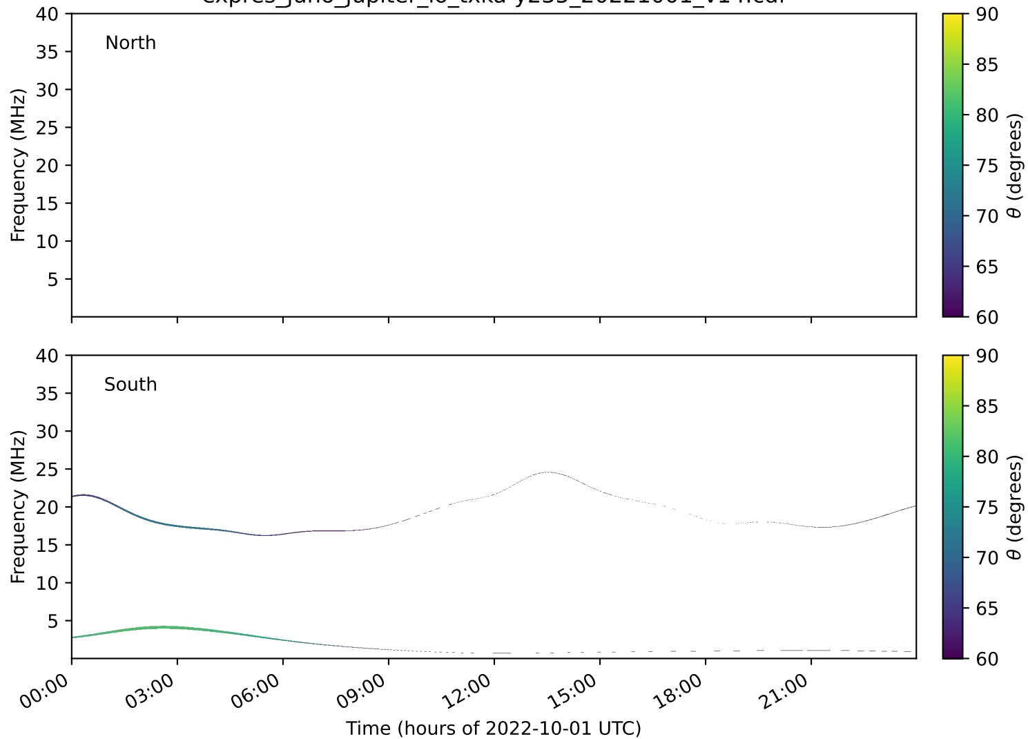
expres_juno_jupiter_io_txka-y235_20221001_v14.cdf
