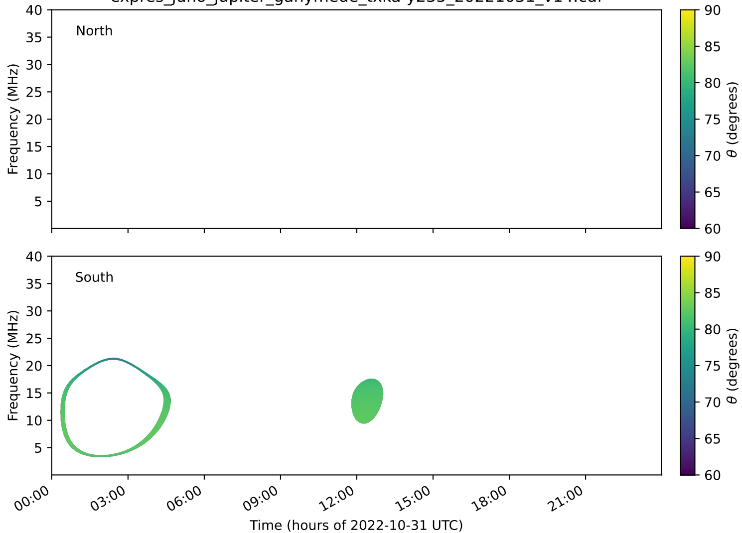
expres_juno_jupiter_ganymede_txka-y235_20221031_v14.cdf
