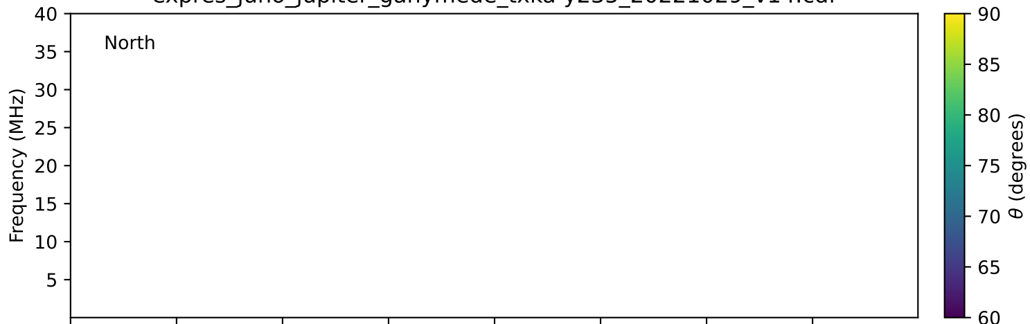
expres_juno_jupiter_ganymede_txka-y235_20221029_v14.cdf
