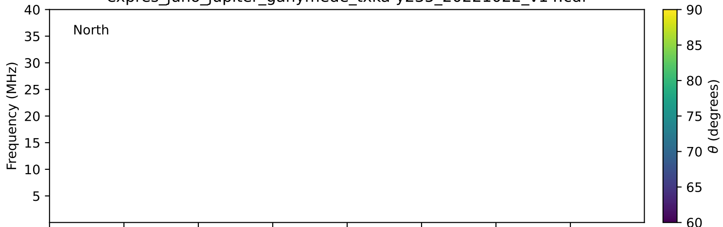
expres_juno_jupiter_ganymede_txka-y235_20221022_v14.cdf
