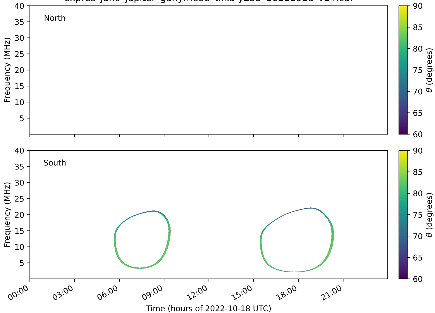
expres_juno_jupiter_ganymede_txka-y235_20221018_v14.cdf
