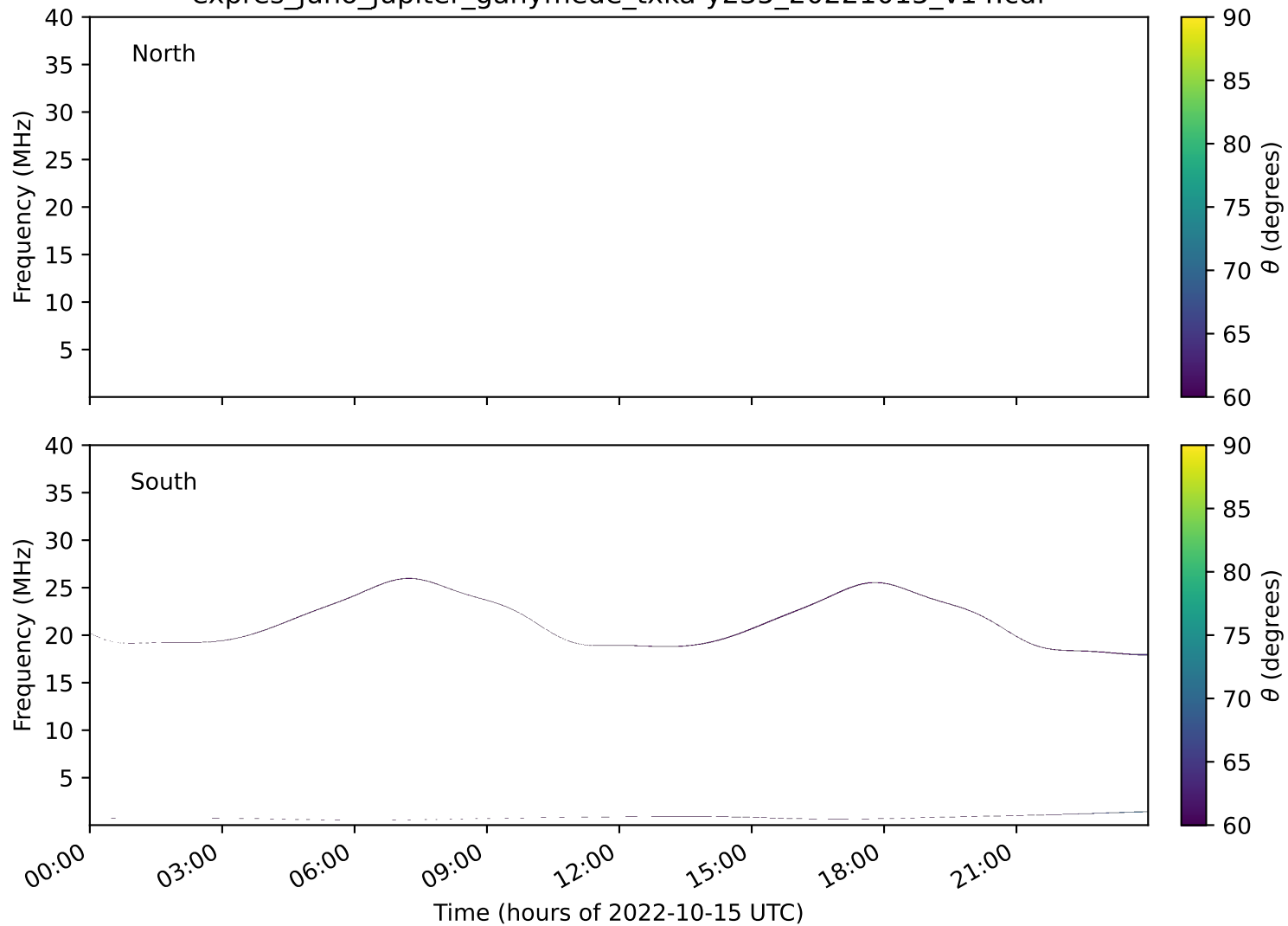
expres_juno_jupiter_ganymede_txka-y235_20221015_v14.cdf
