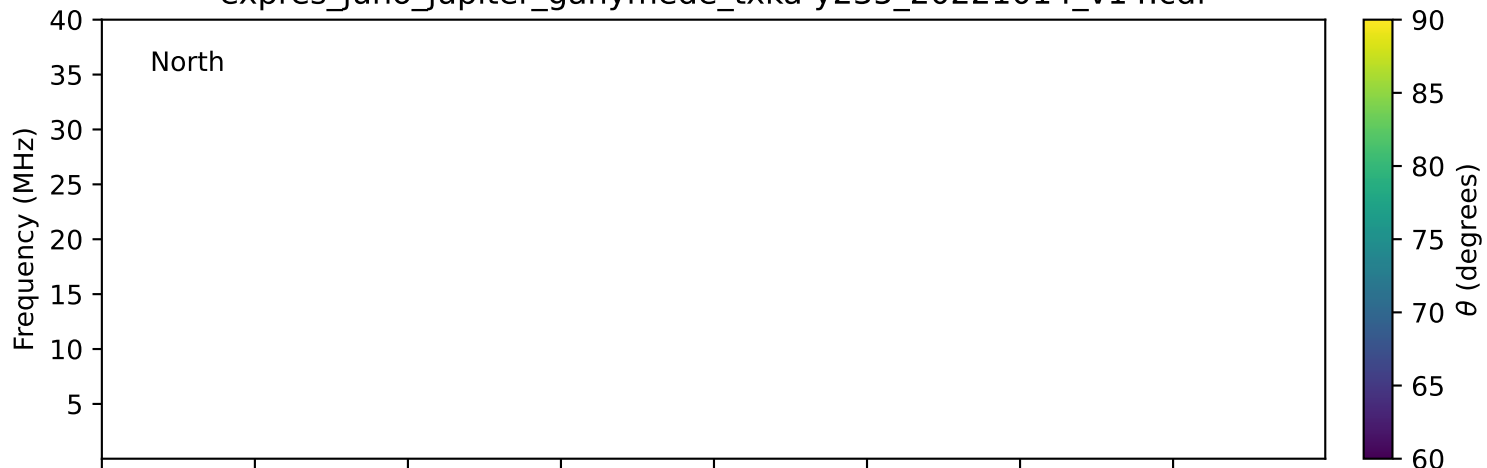
expres_juno_jupiter_ganymede_txka-y235_20221014_v14.cdf
