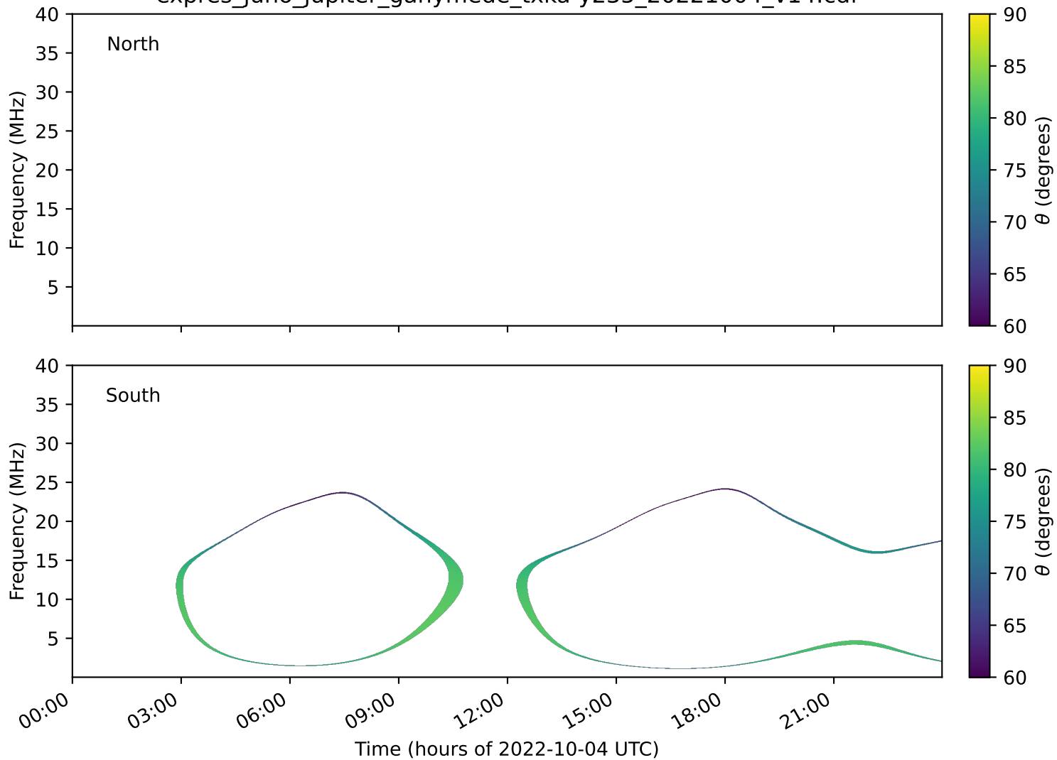
expres_juno_jupiter_ganymede_txka-y235_20221004_v14.cdf
