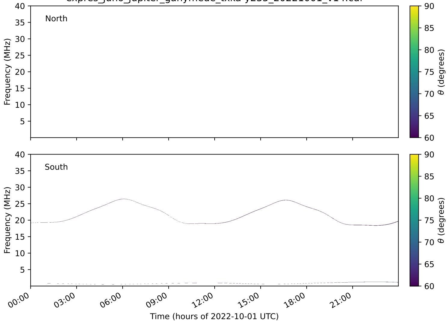
expres_juno_jupiter_ganymede_txka-y235_20221001_v14.cdf
