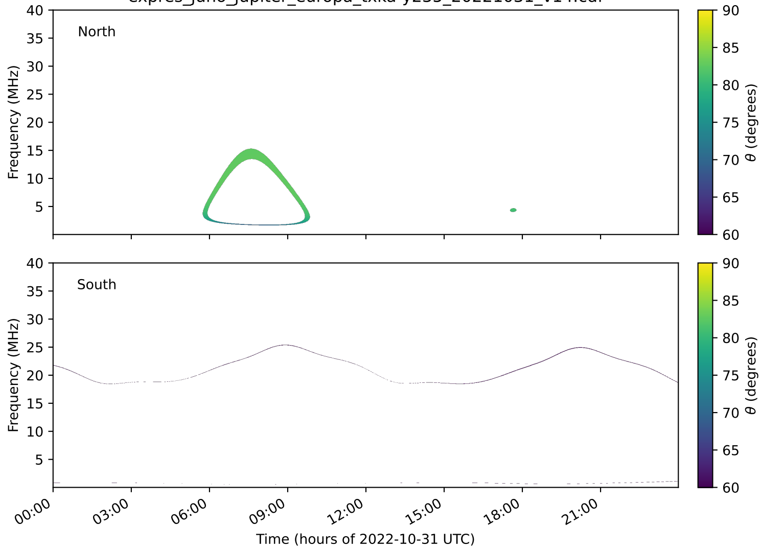
expres_juno_jupiter_europa_txka-y235_20221031_v14.cdf
