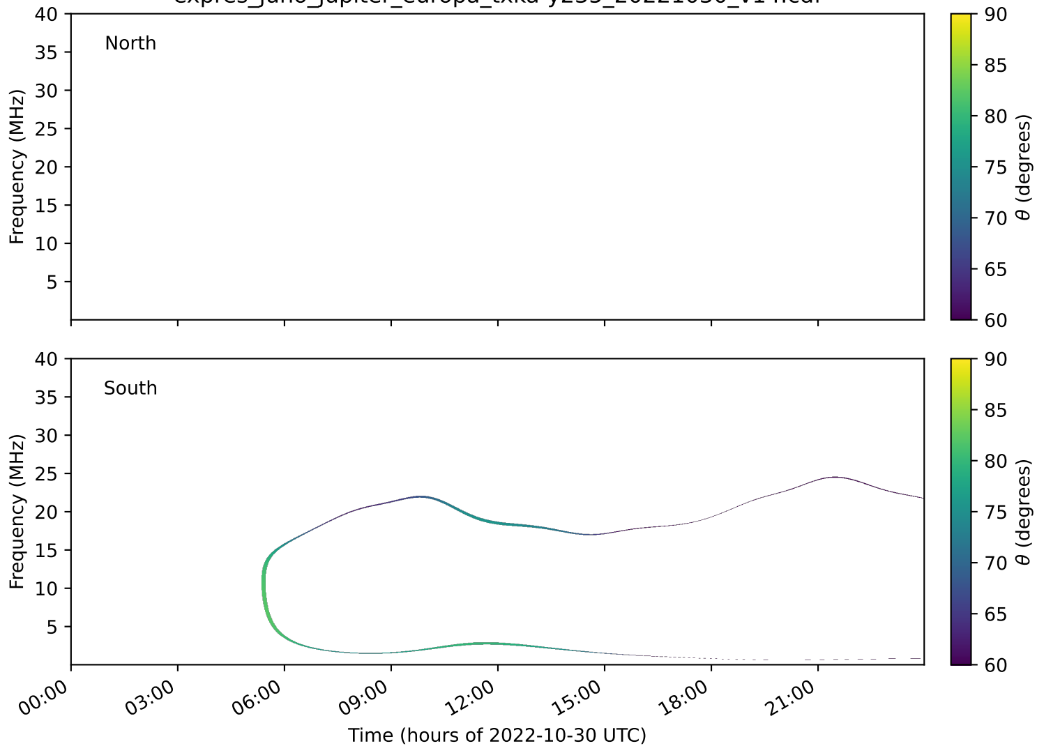
expres_juno_jupiter_europa_txka-y235_20221030_v14.cdf
