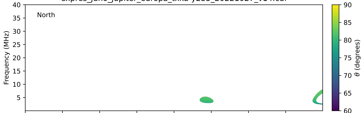
expres_juno_jupiter_europa_txka-y235_20221027_v14.cdf
