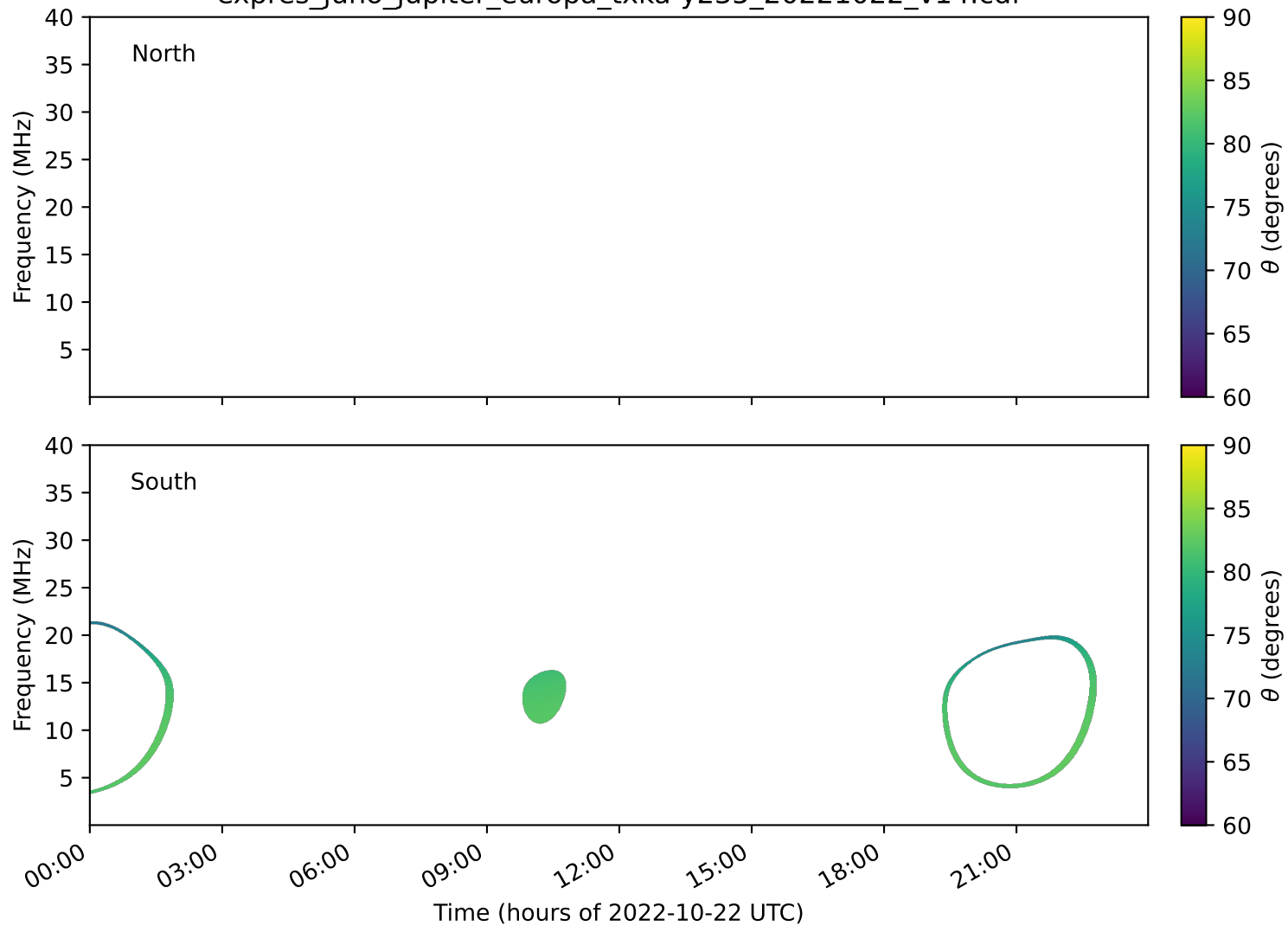
expres_juno_jupiter_europa_txka-y235_20221022_v14.cdf
