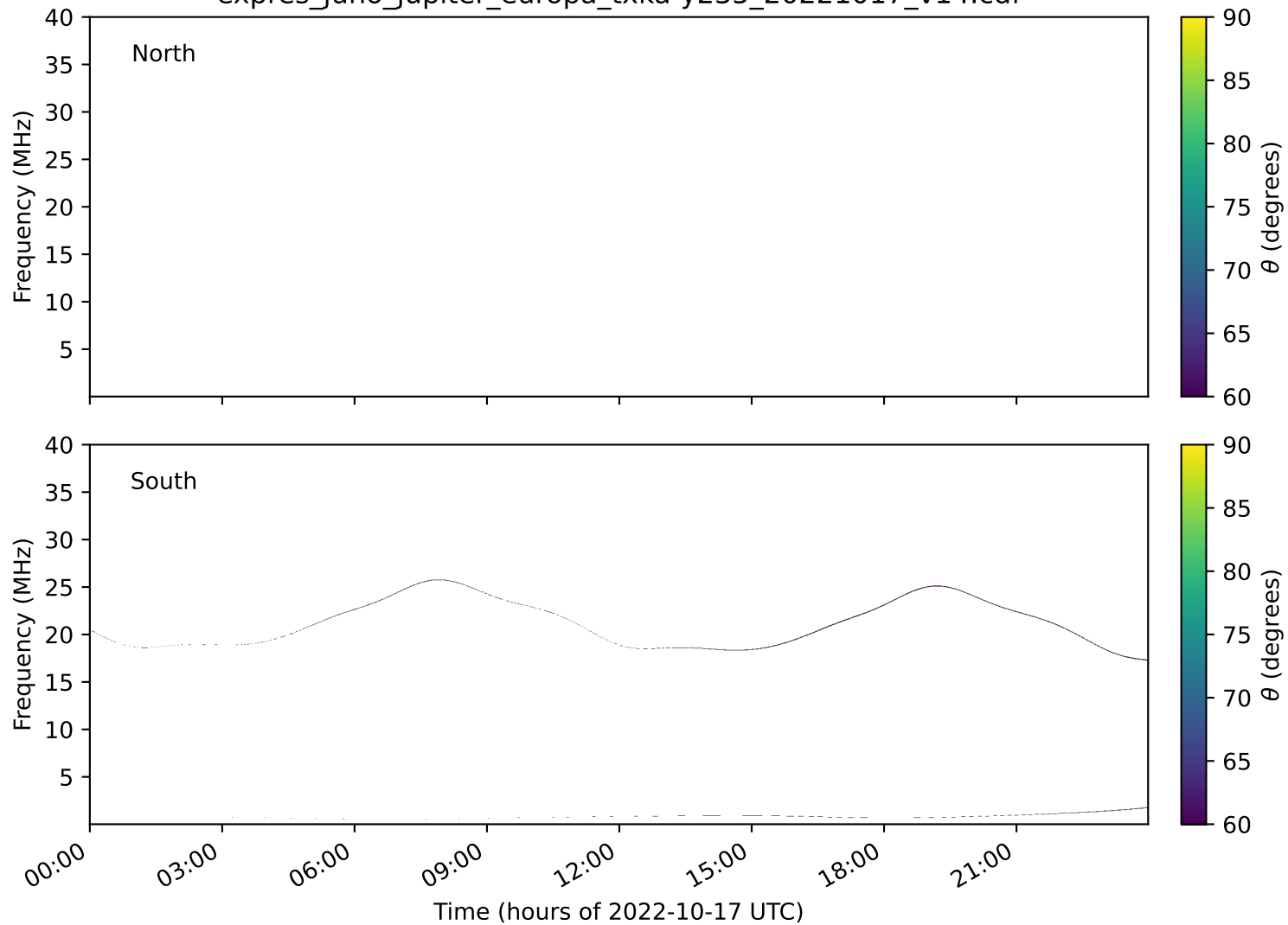
expres_juno_jupiter_europa_txka-y235_20221017_v14.cdf
