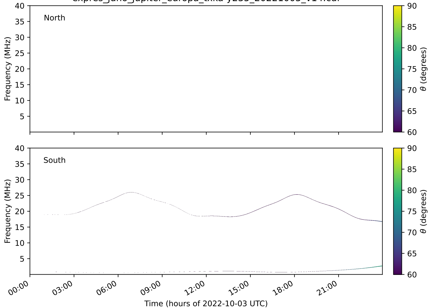
expres_juno_jupiter_europa_txka-y235_20221003_v14.cdf
