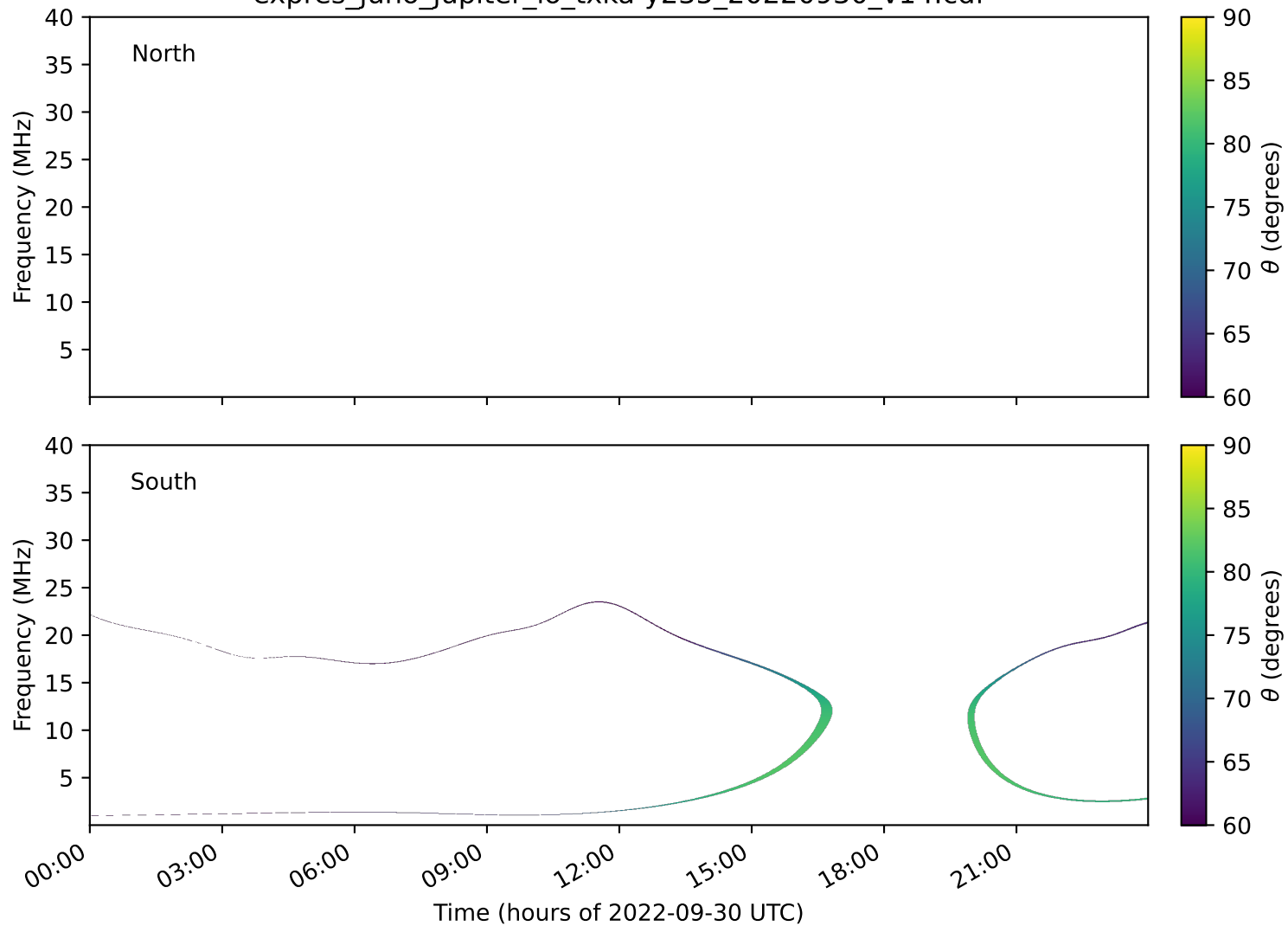
expres_juno_jupiter_io_txka-y235_20220930_v14.cdf
