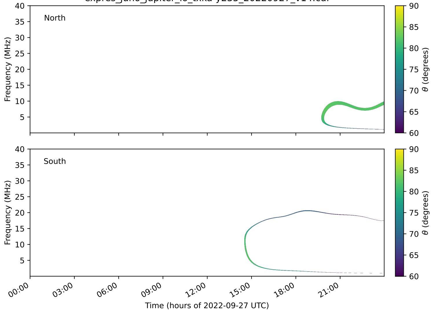
expres_juno_jupiter_io_txka-y235_20220927_v14.cdf
