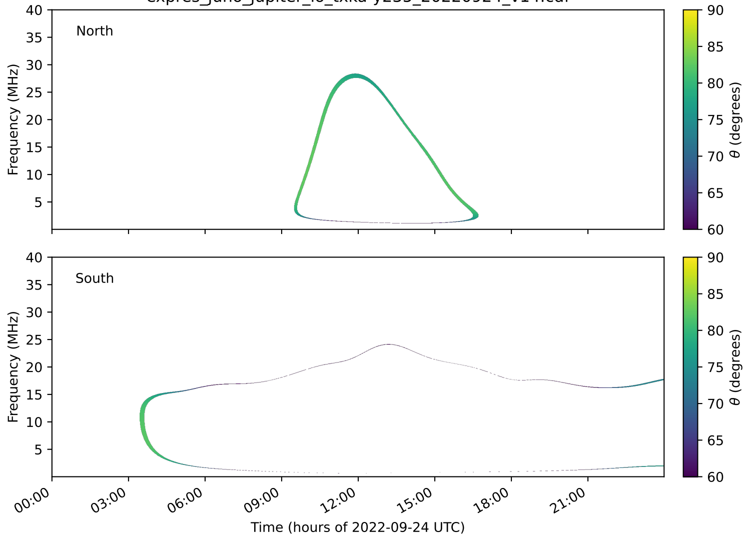
expres_juno_jupiter_io_txka-y235_20220924_v14.cdf
