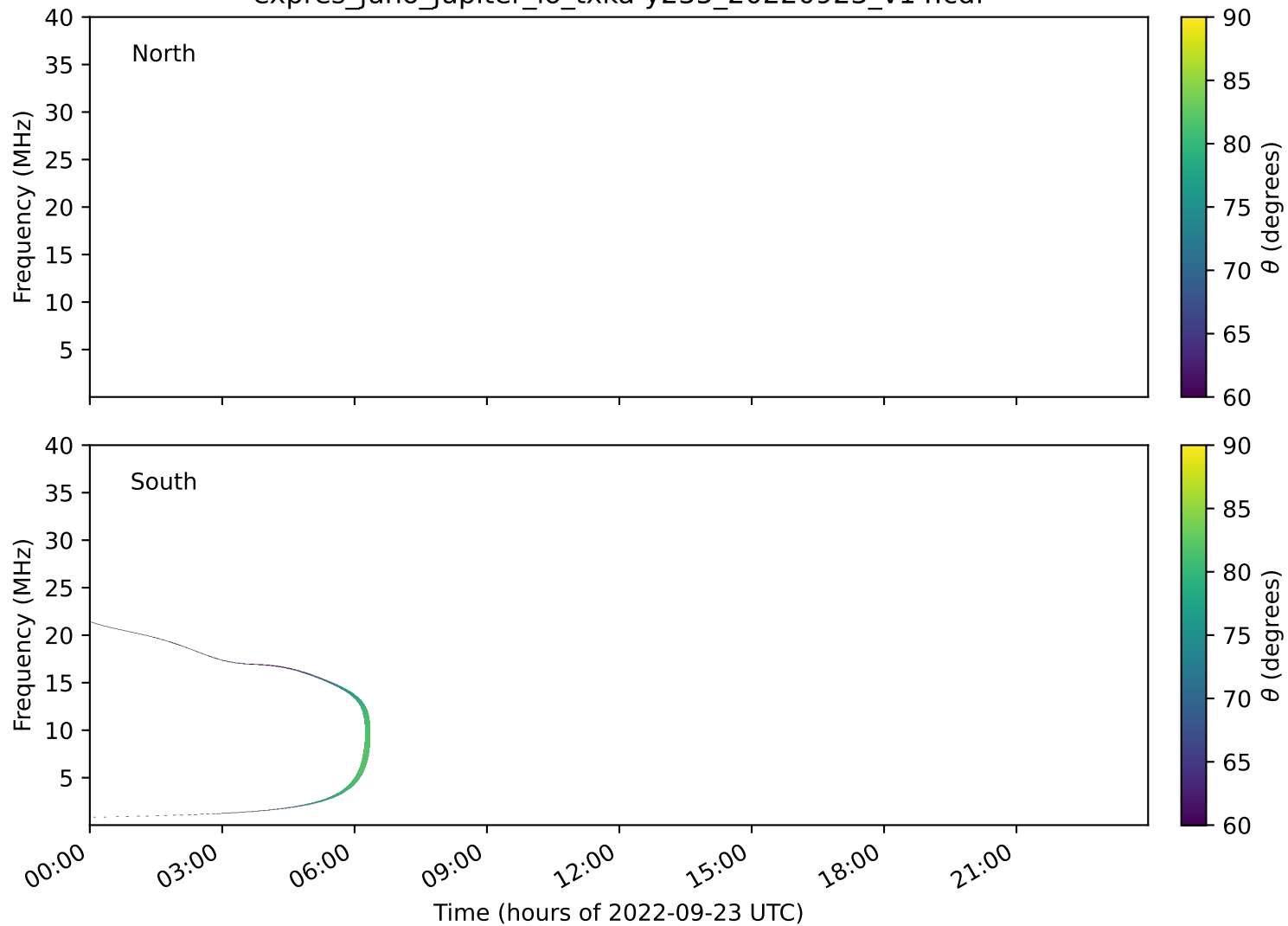
expres_juno_jupiter_io_txka-y235_20220923_v14.cdf
