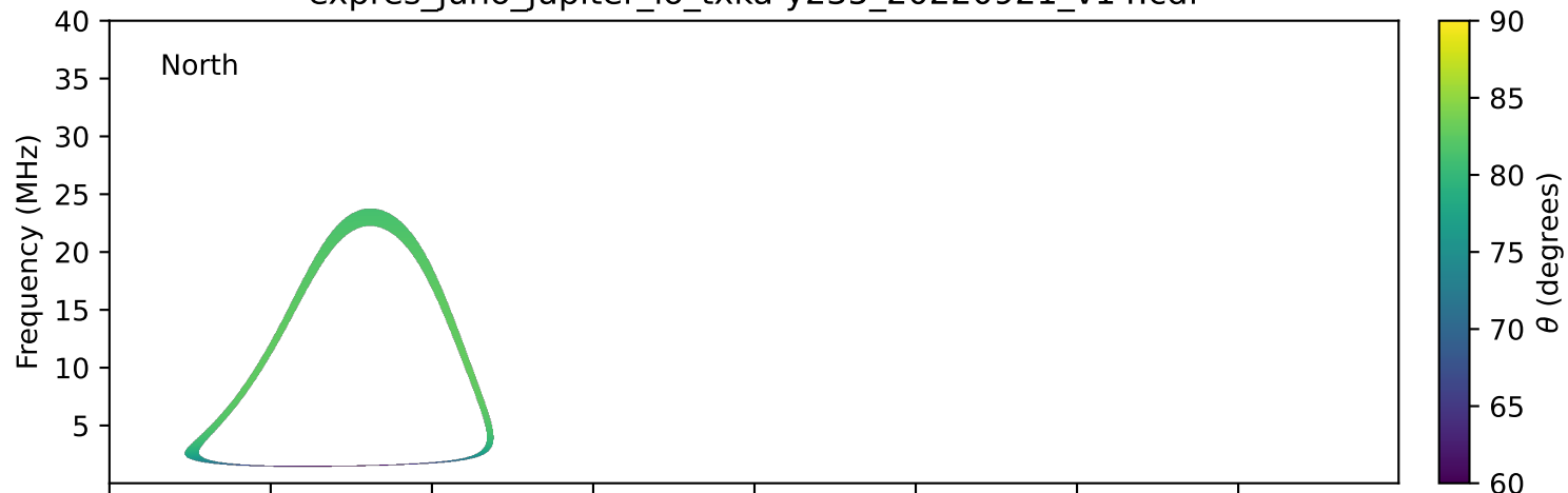
expres_juno_jupiter_io_txka-y235_20220921_v14.cdf
