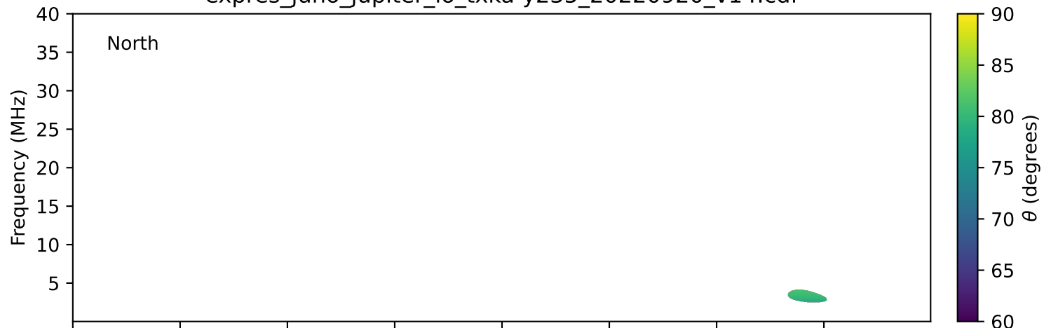
expres_juno_jupiter_io_txka-y235_20220920_v14.cdf
