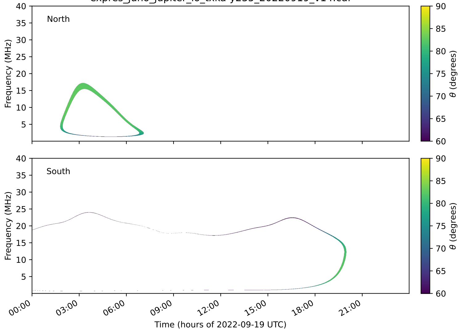
expres_juno_jupiter_io_txka-y235_20220919_v14.cdf
