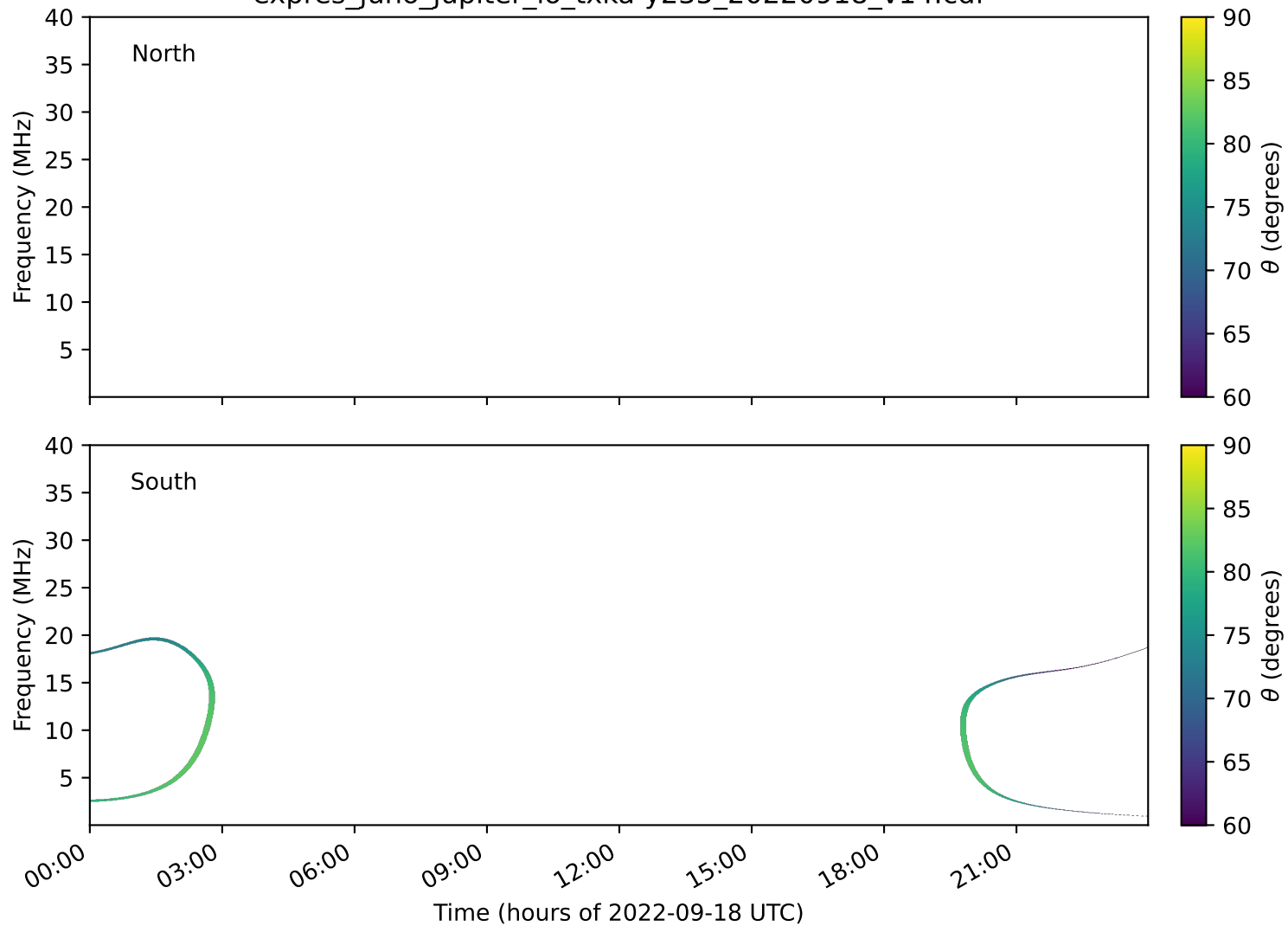
expres_juno_jupiter_io_txka-y235_20220918_v14.cdf
