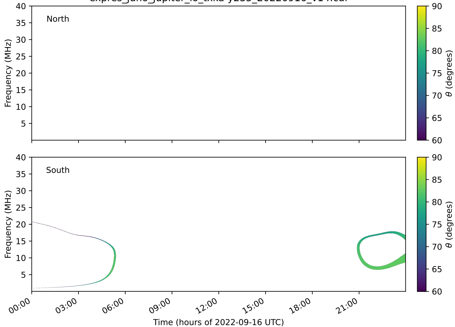
expres_juno_jupiter_io_txka-y235_20220916_v14.cdf
