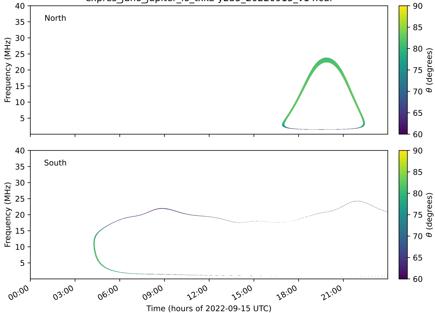
expres_juno_jupiter_io_txka-y235_20220915_v14.cdf
