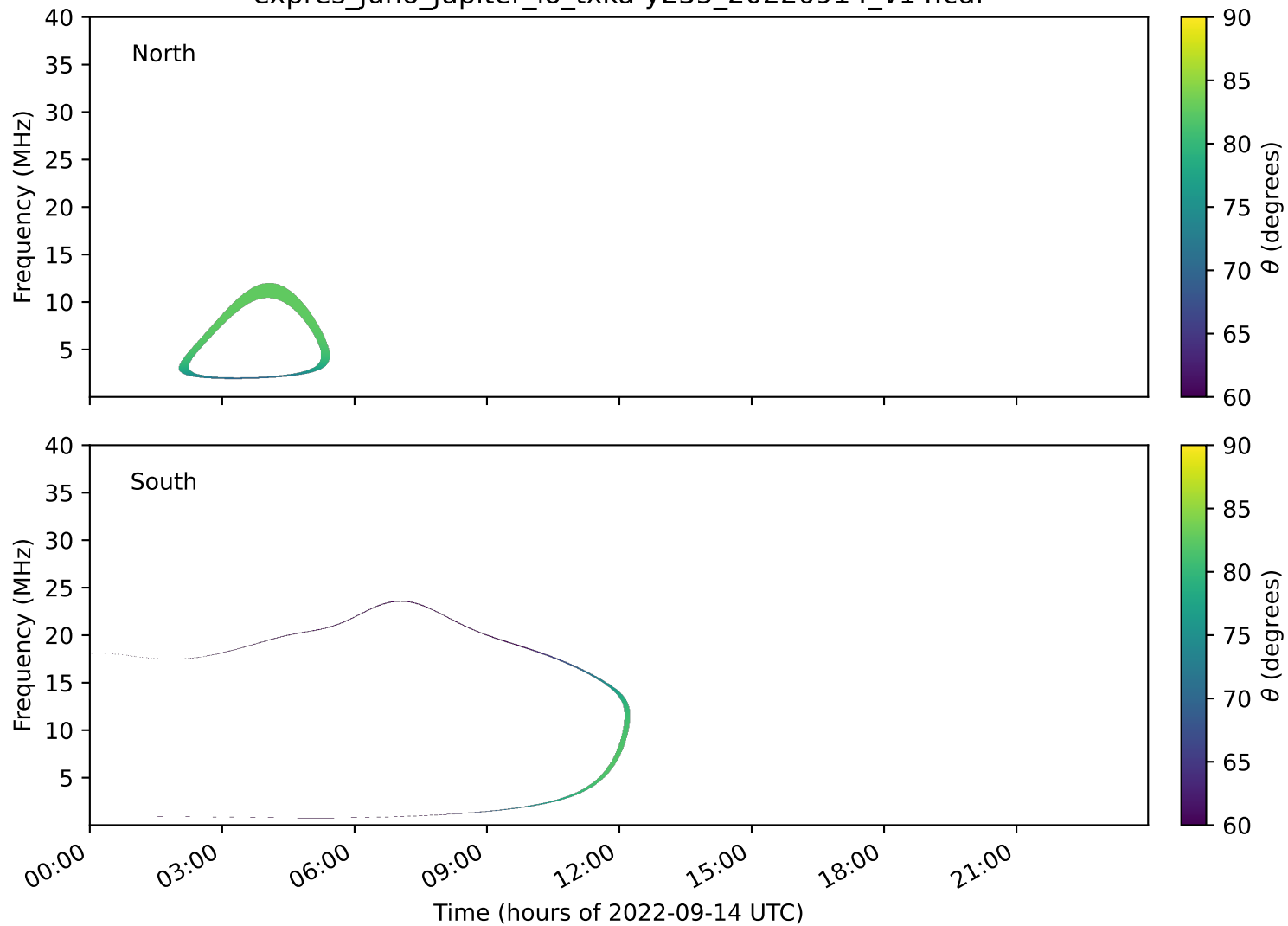
expres_juno_jupiter_io_txka-y235_20220914_v14.cdf
