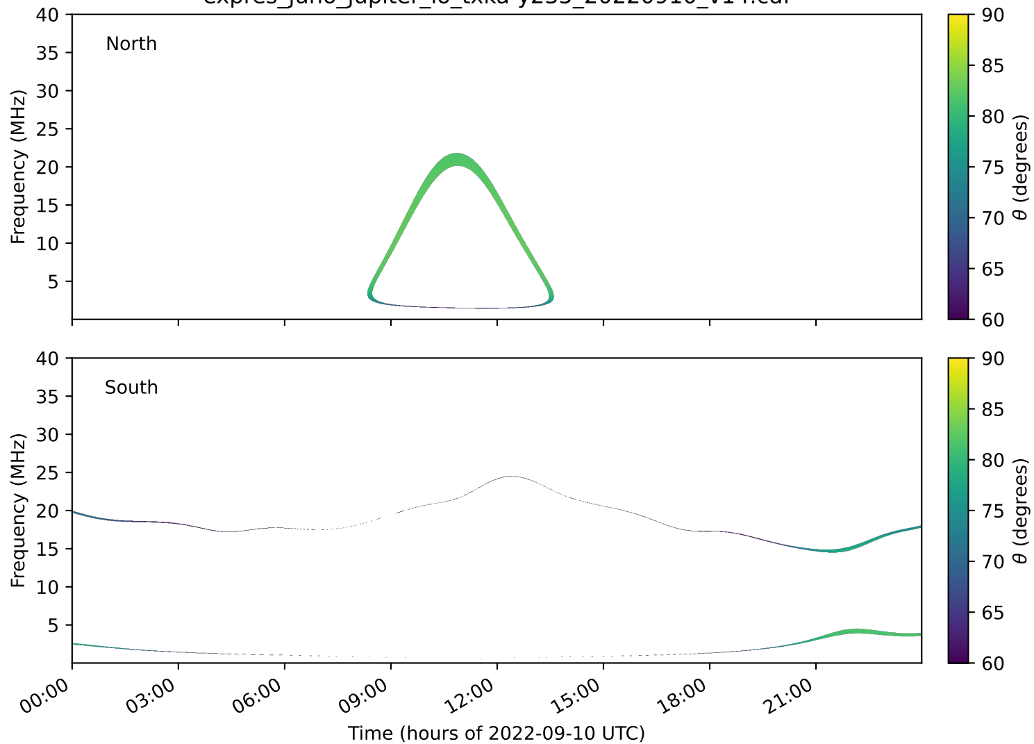
expres_juno_jupiter_io_txka-y235_20220910_v14.cdf
