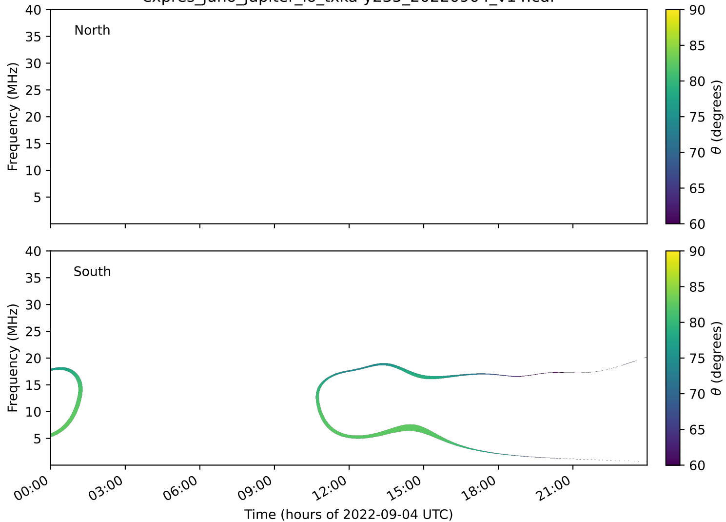
expres_juno_jupiter_io_txka-y235_20220904_v14.cdf
