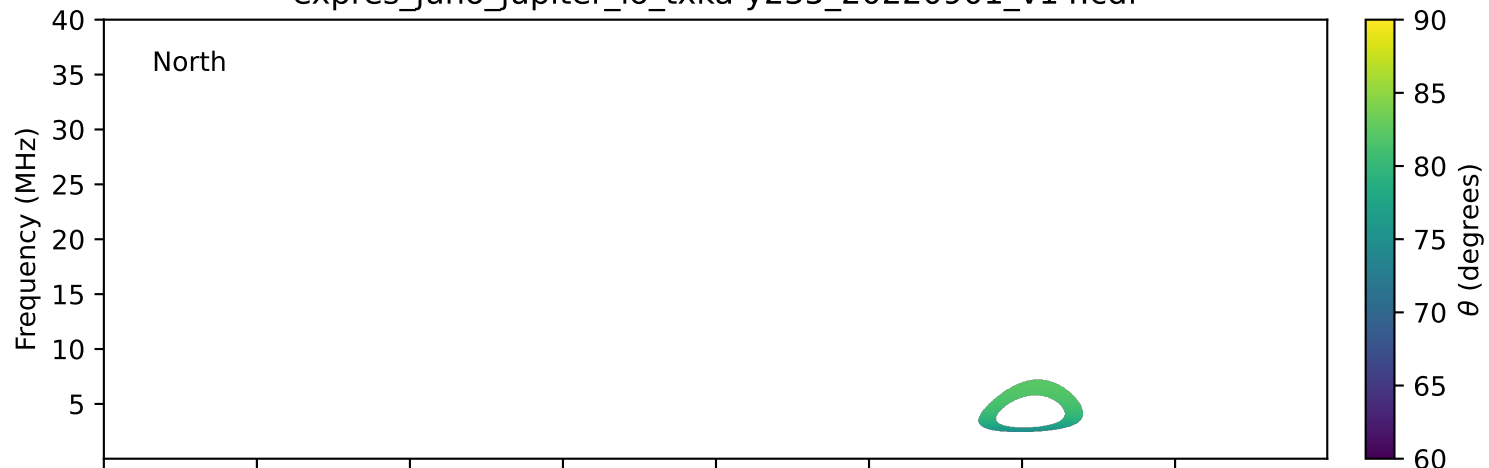
expres_juno_jupiter_io_txka-y235_20220901_v14.cdf
