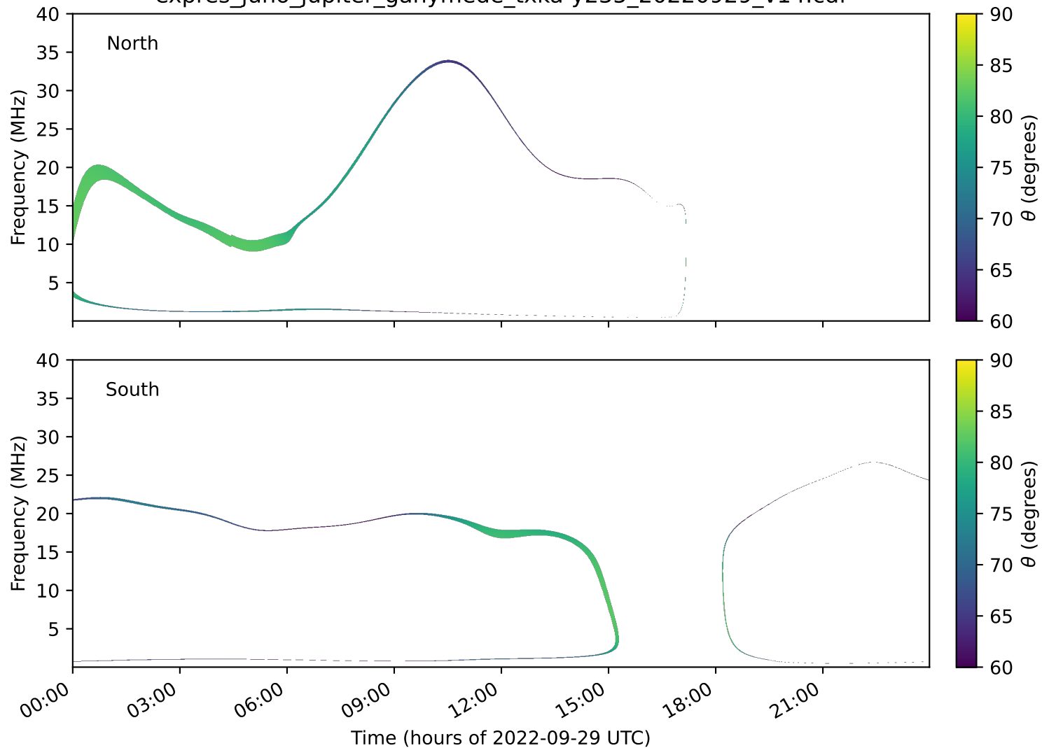
expres_juno_jupiter_ganymede_txka-y235_20220929_v14.cdf
