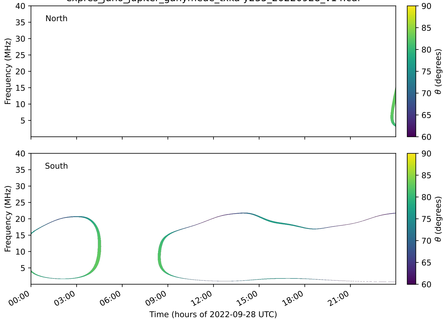
expres_juno_jupiter_ganymede_txka-y235_20220928_v14.cdf
