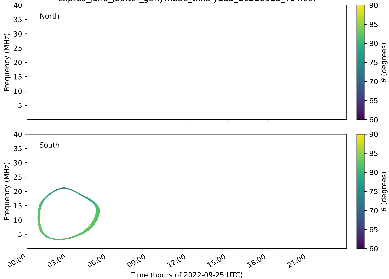
expres_juno_jupiter_ganymede_txka-y235_20220925_v14.cdf
