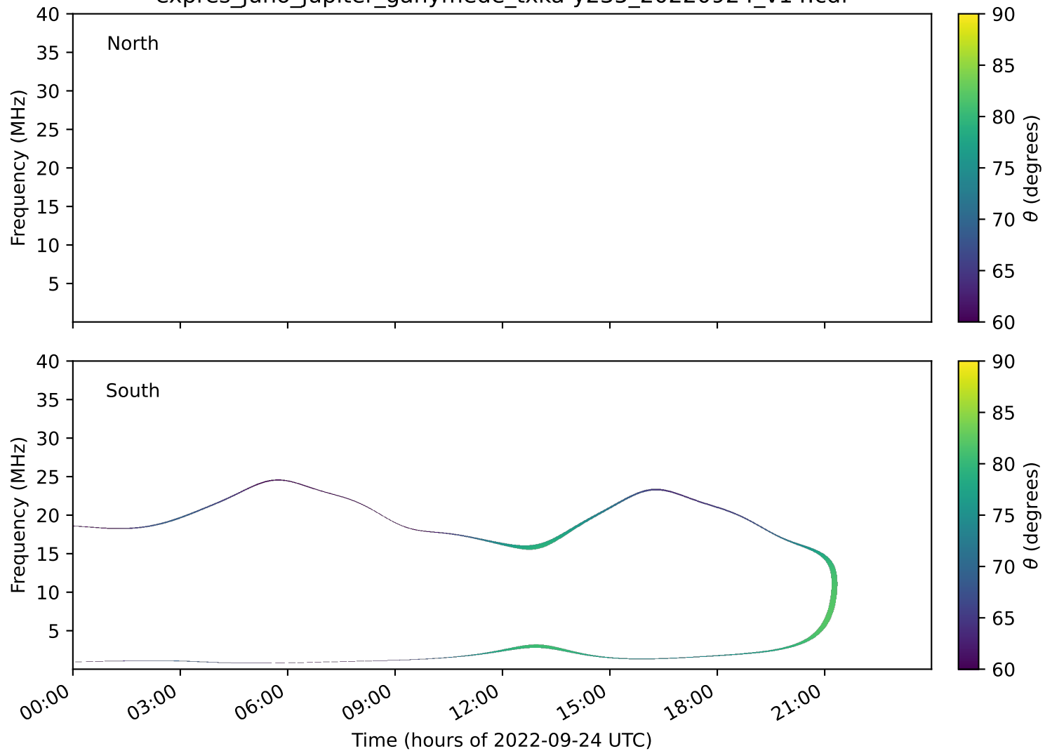
expres_juno_jupiter_ganymede_txka-y235_20220924_v14.cdf
