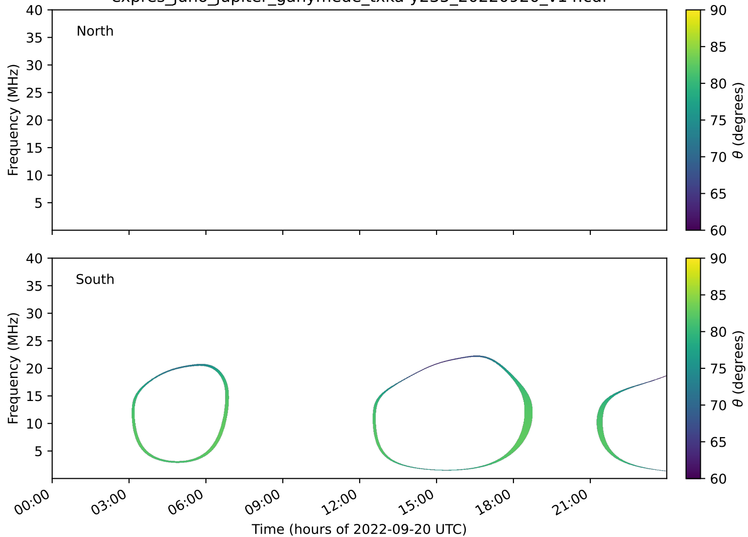
expres_juno_jupiter_ganymede_txka-y235_20220920_v14.cdf
