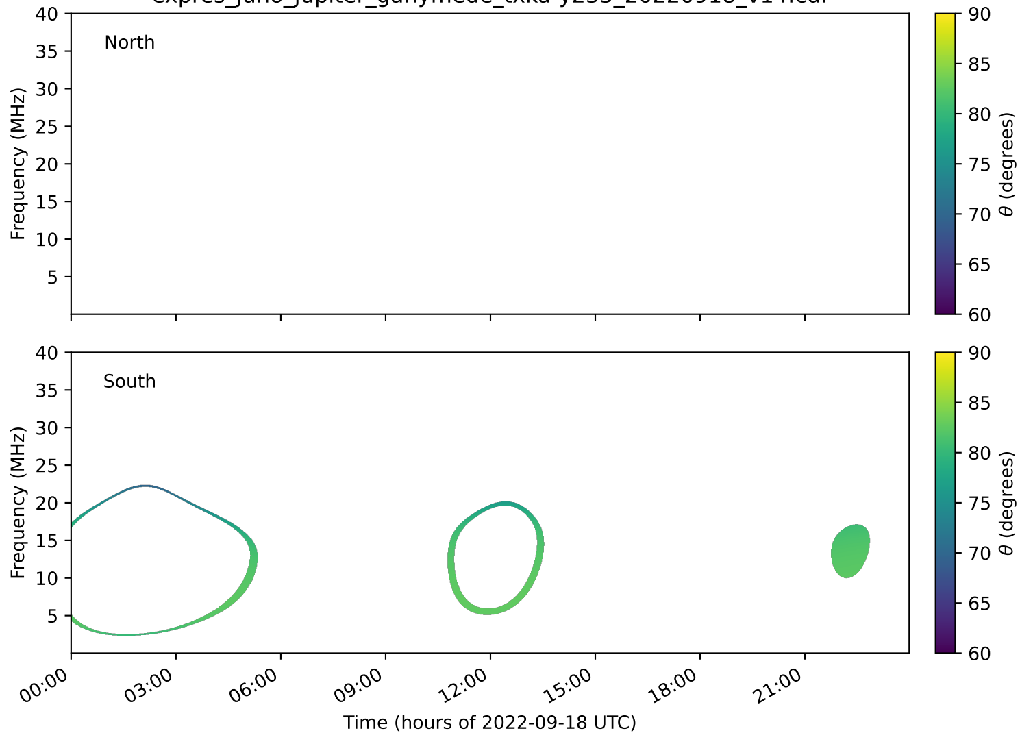
expres_juno_jupiter_ganymede_txka-y235_20220918_v14.cdf
