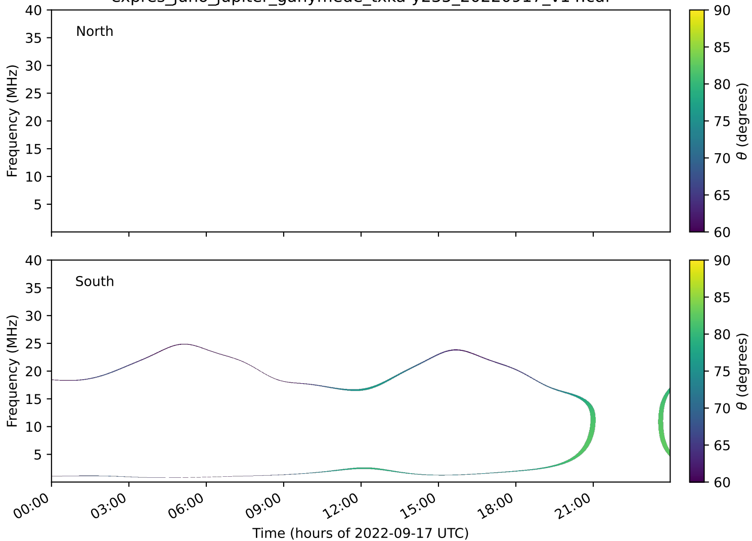
expres_juno_jupiter_ganymede_txka-y235_20220917_v14.cdf
