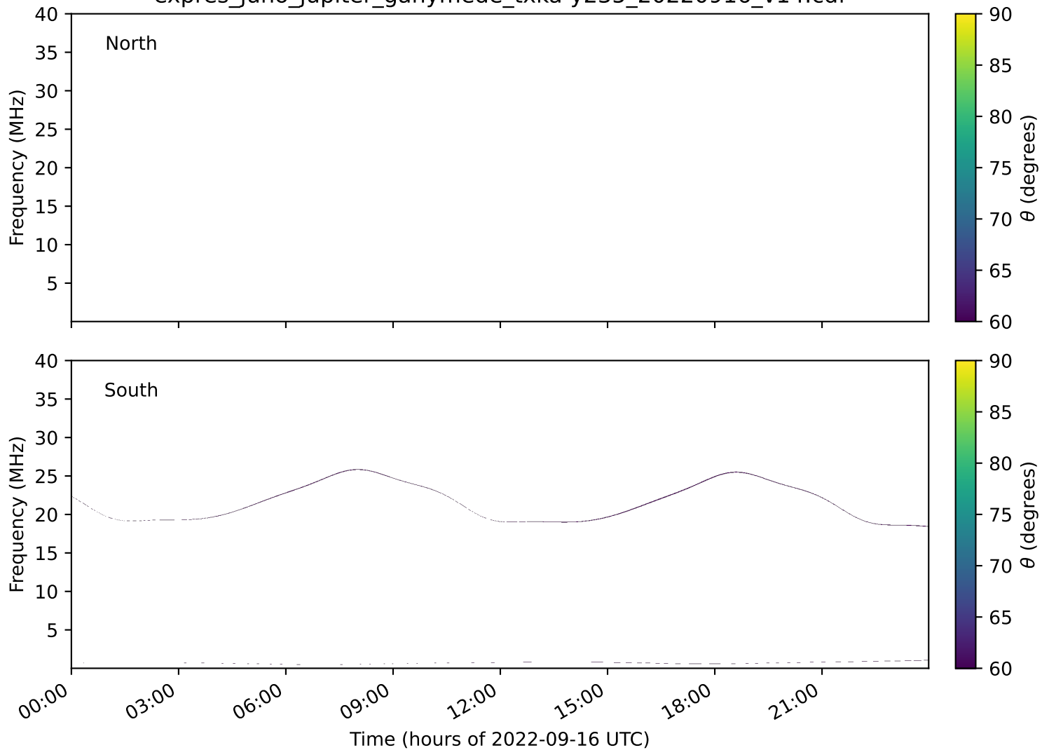
expres_juno_jupiter_ganymede_txka-y235_20220916_v14.cdf
